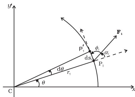
Fig. 6.30 Work done by a force \mathbf{F}_1 acting on a particle of a body rotating about a fixed axis; the particle describes a circular path with centre C on the axis; arc P_1P'_1 ( ds_1 ) gives the displacement of the particle.
